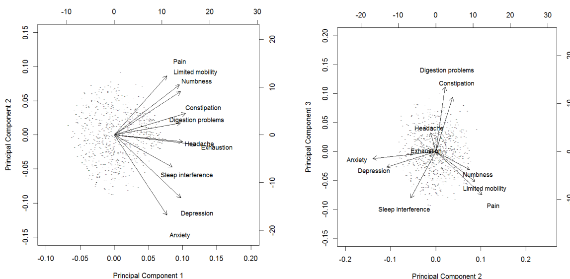
Figure 1. Biplots between principal components 1 and 2, 2 and 3.
